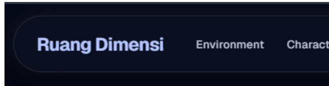
IMG 6 Logo
