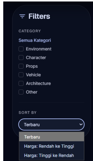
IMG 8 Filter
