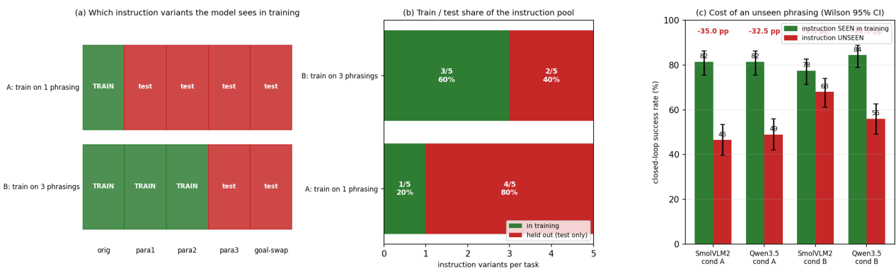
Figure 4. (a) which instruction variants each condition trains on; (b) train/test share of the instruction pool (20% vs 60%); (c) closed-loop cost of an unseen phrasing, both backbones, Wilson 95% CI.
