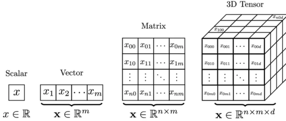
Figure 2.1: Examples of rank-0, 1, 2, 3 tensors (i.e. a scalar, vector, matrix, order-3 tensor). Adapted from [5].
