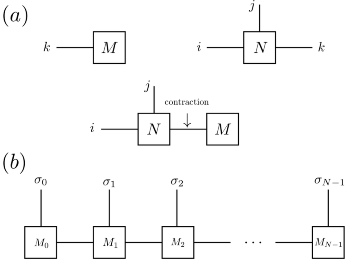
Figure 2.2.: (a), on the top, displays a vector, M , and a rank-3 tensor, N , contracted across their common leg k ; (b), on the bottom, displays a complex network of N tensors chained in a tensor train, commonly known as a Matrix Product State (MPS)
