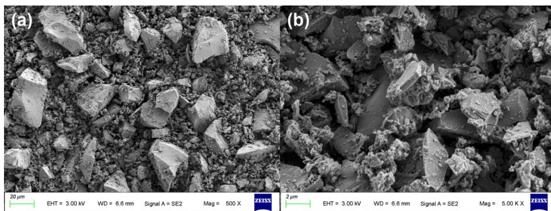
Figure S4. SEM micrographs of sample B2 (10 min). Left: 500×; right: 5,000×. The scale bars are 20 μm and 2 μm, respectively.
