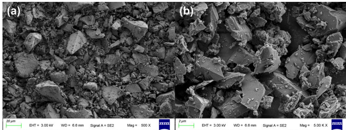
Figure S2. SEM micrographs of the as-received GGBS sample B0 (0 min). Left: 500 \times ; right: 5,000 \times . The scale bars are 20 \mu\text{m} and 2 \mu\text{m} , respectively.
