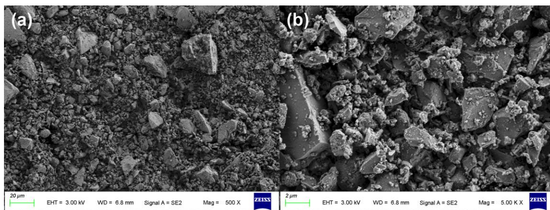
Figure S8. SEM micrographs of sample B6 (30 min). Left: 500×; right: 5,000×. The scale bars are 20 μm and 2 μm, respectively.
