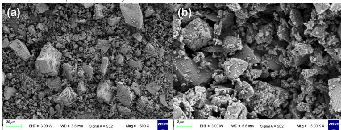
Figure S5. SEM micrographs of sample B3 (15 min). Left: 500×; right: 5,000×. The scale bars are 20 μm and 2 μm, respectively.
