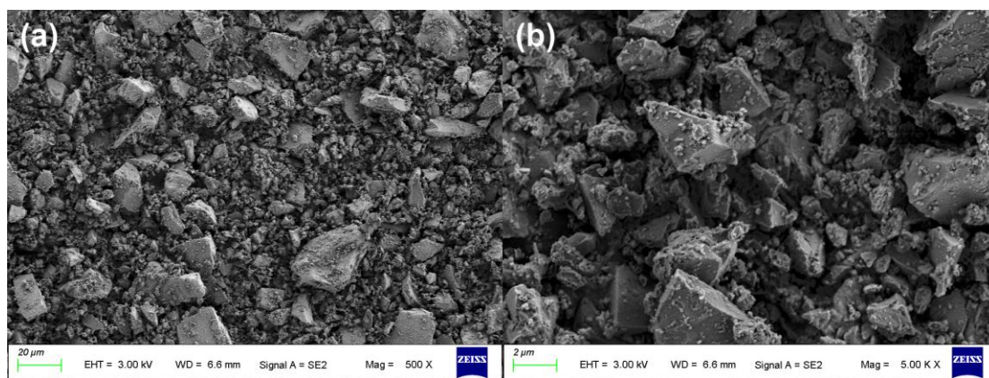
Figure S6. SEM micrographs of sample B4 (20 min). Left: 500×; right: 5,000×. The scale bars are 20 μm and 2 μm, respectively.
