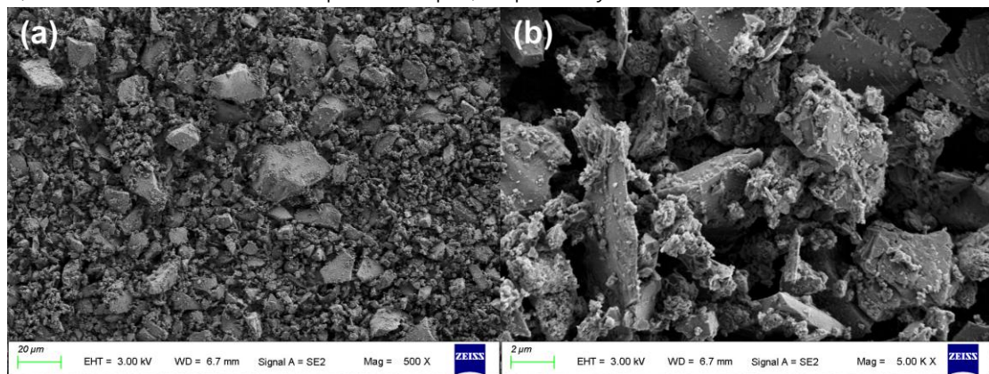
Figure S3. SEM micrographs of sample B1 (5 min). Left: 500 \times ; right: 5,000 \times . The scale bars are 20 \mu\text{m} and 2 \mu\text{m} , respectively.
