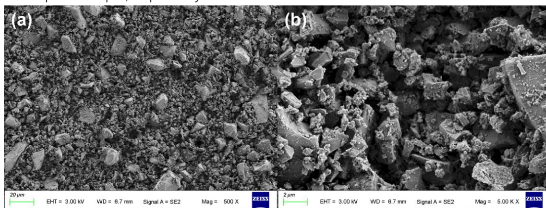
Figure S9. SEM micrographs of sample B7 (35 min). Left: 500×; right: 5,000×. The scale bars are 20 μm and 2 μm, respectively.
