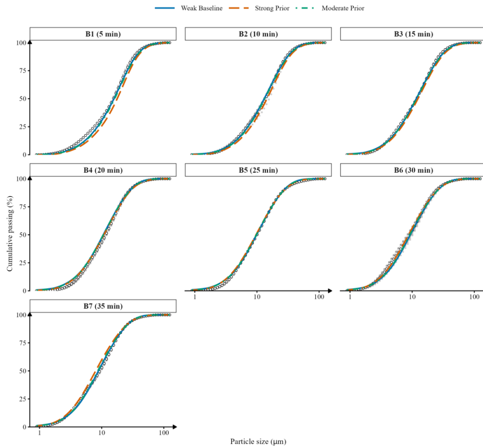
Figure S1. Observed cumulative particle-size distributions (PSDs) for B1–B7 and posterior-median predictions under the three prior scenarios. Grey points show the six experimental replicates, white-filled points and grey bands show their pointwise mean \pm 1 standard deviation, and colored lines show the mean of the six replicate-specific posterior-median fitted curves.
