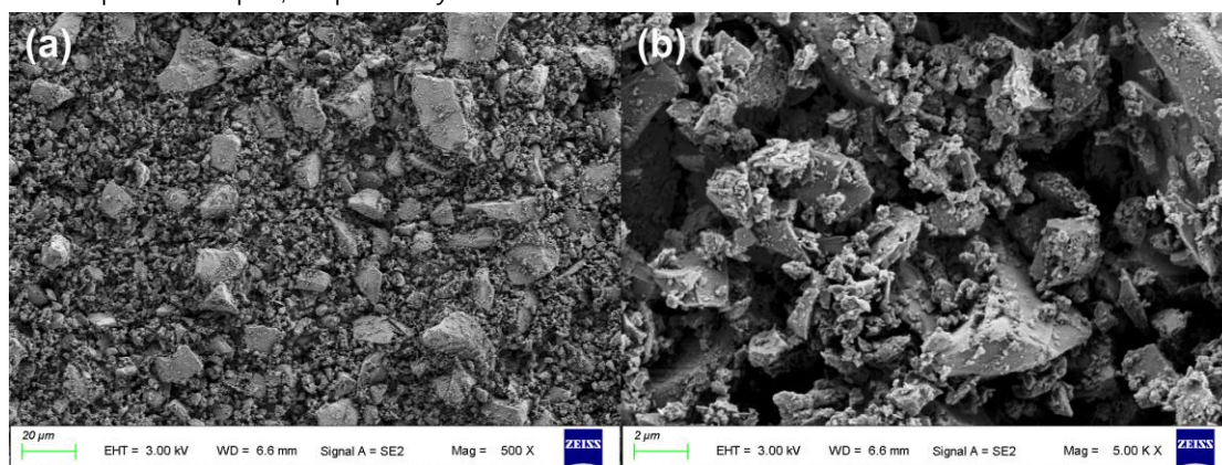
Figure S7. SEM micrographs of sample B5 (25 min). Left: 500×; right: 5,000×. The scale bars are 20 μm and 2 μm, respectively.
