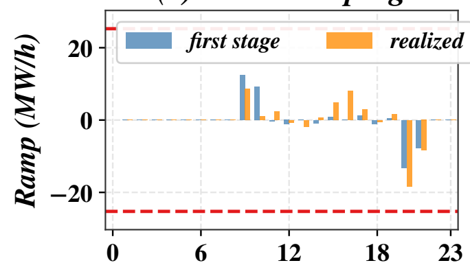
(e) Gen 7 ramping
