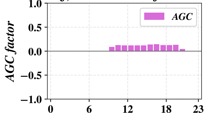
(f) Gen 19 AGC factor
