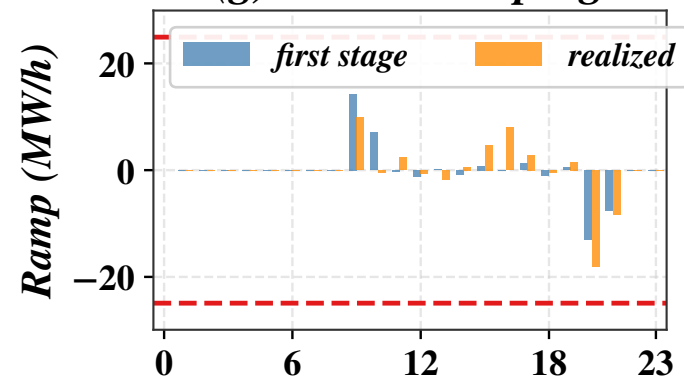
(g) Gen 19 ramping
