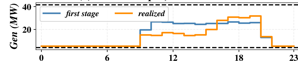
(c) Gen 19 output, 52.62 USD/MWh
