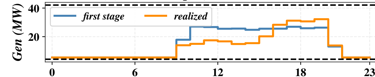
(b) Gen 7 output, 53.36 USD/MWh
