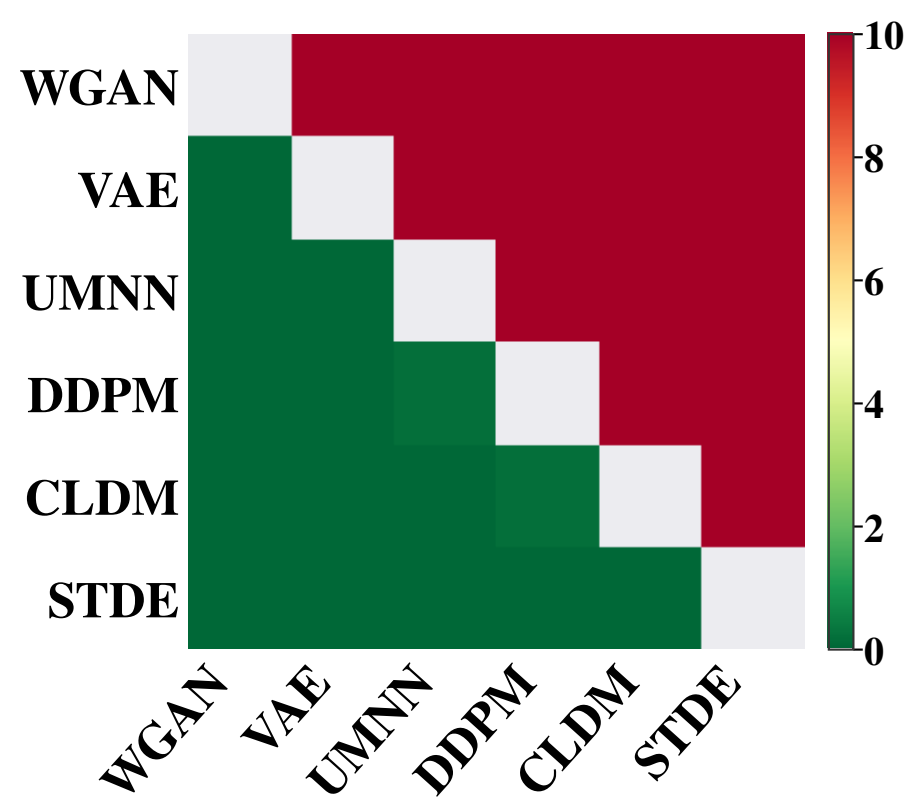
(a) CRPS DM test.
