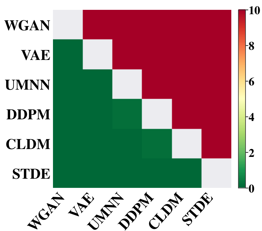
(b) PS DM test.
