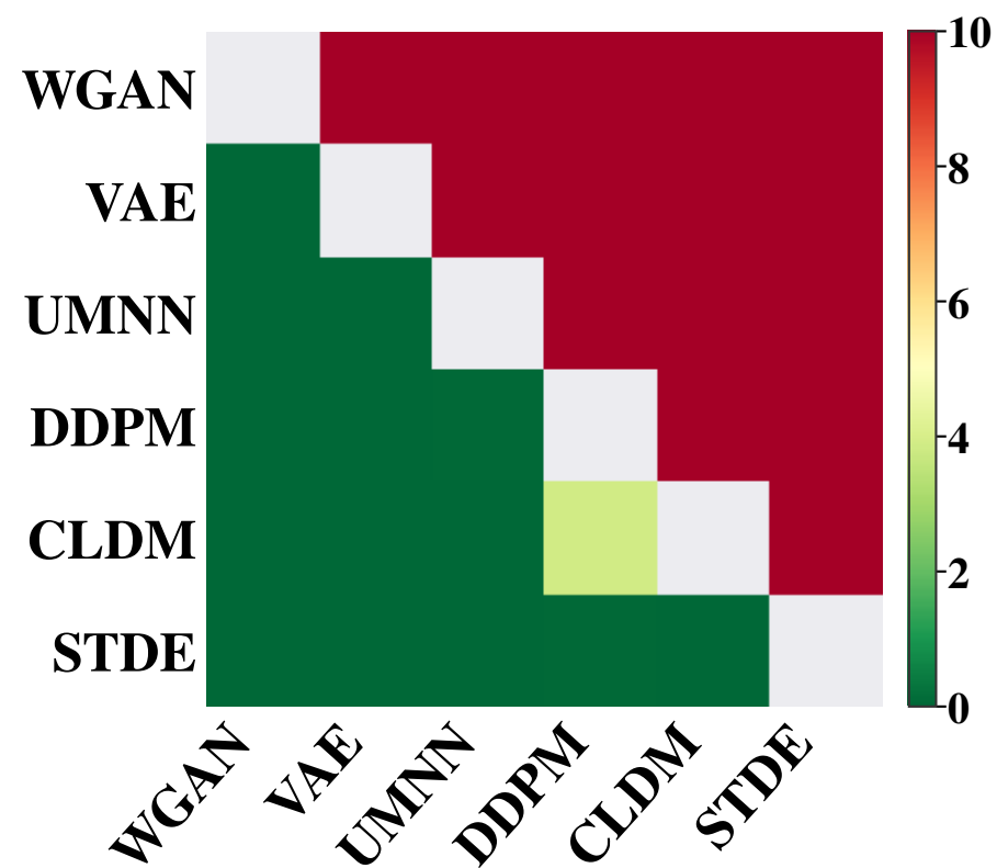
(c) ES DM test.
