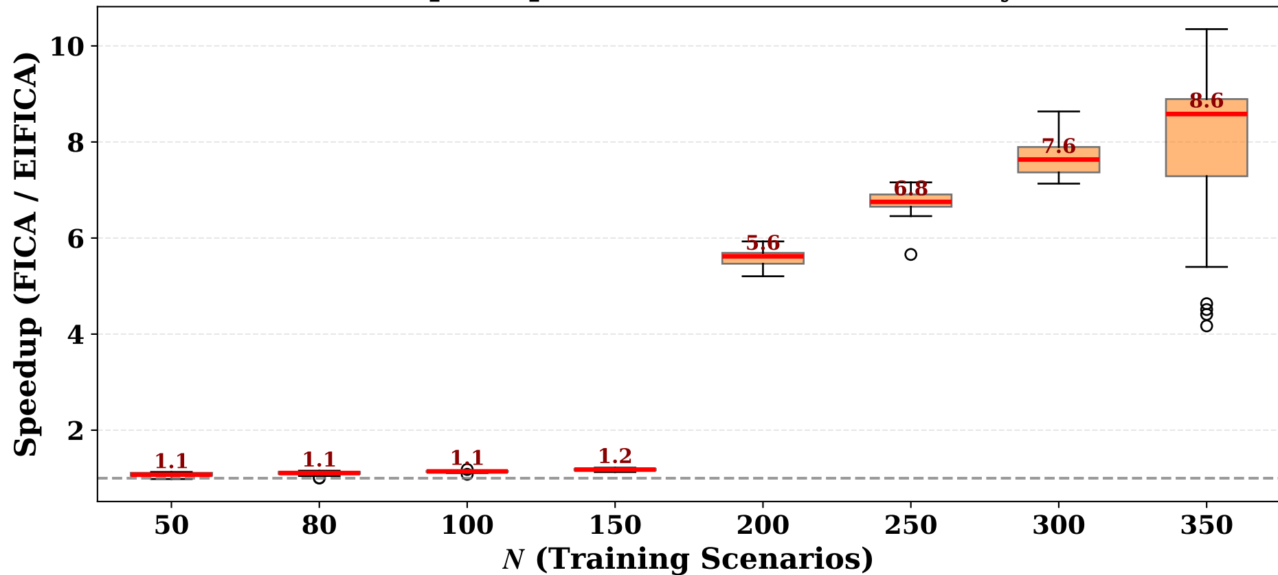
EIFICA Speedup over FICA IEEE 118-Bus System
