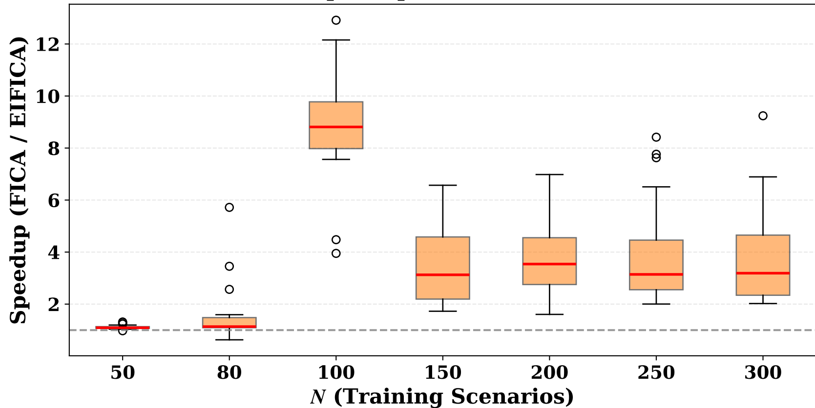
EIFICA Speedup over FICA (with ESS)
