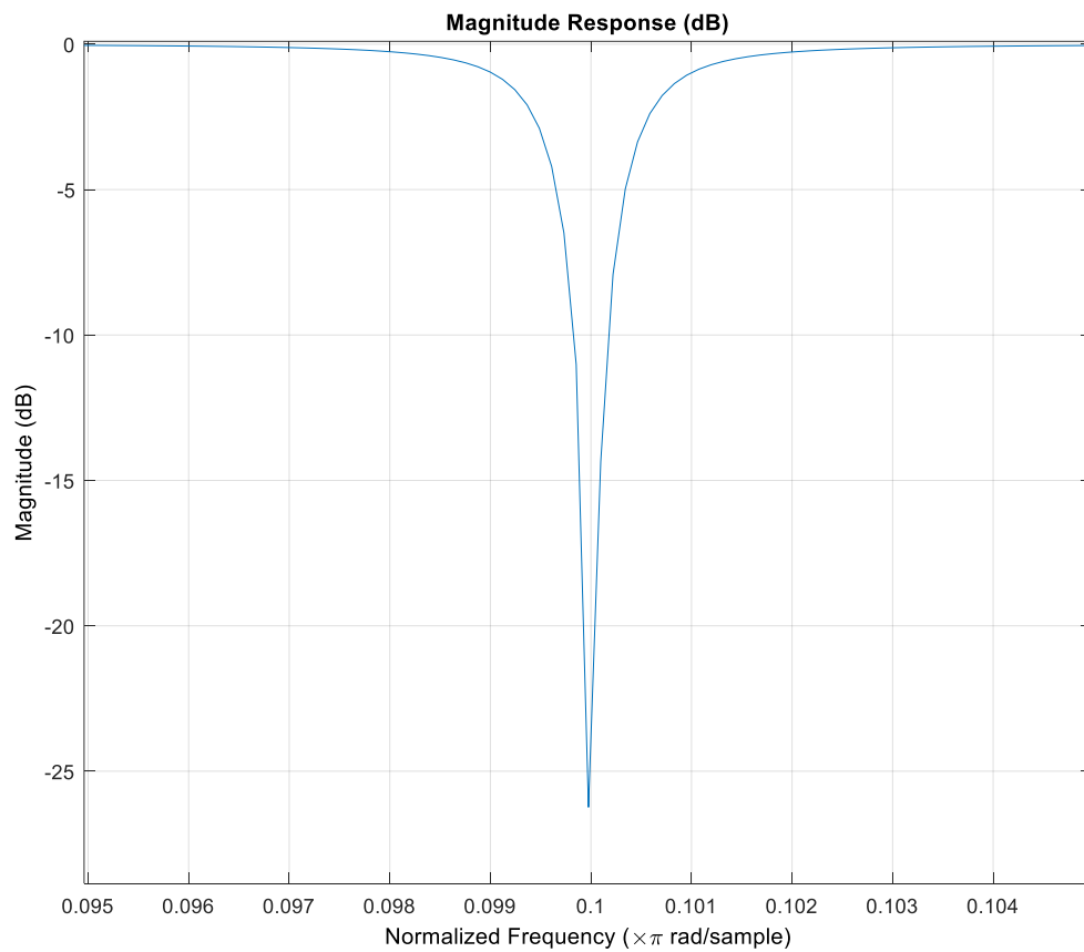
圖(一)、magnitude response of IIR notch filter
