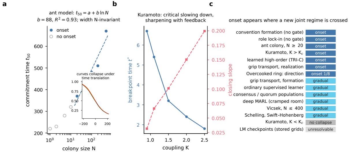
Figure 6. Scaling and scope. a , Finite-size scaling in the ant model: commitment time is consistent with t_{50} = a + b \ln N ( b = 88 , 95% CI [41, 124], R^2 = 0.93 ; dashed fit), as predicted by nucleation from N^{-1/2} fluctuations; open circles, sizes below the onset threshold. Inset: median collapse curves for N = 50 –500 superpose under pure time translation (aligned RMS 0.010 vs 0.266 unaligned)—the profile is universal, only the timing shifts. b , Kuramoto criticality: breakpoint time falls and closing slope rises as coupling increases; subcritical runs are gated null. c , Classification: onset appears where a joint-regime barrier is crossed—including without any designed gate (convention formation, role lock-in) and in the standard Overcooked coordination-ring layout, where all 8 seeds commit to a circulation direction and 1/8 certifies onset (Results)—and is absent for gradual convergence (formation, ordinary learners, consensus/quorum populations, cramped-room deep MARL, several classic cases).
