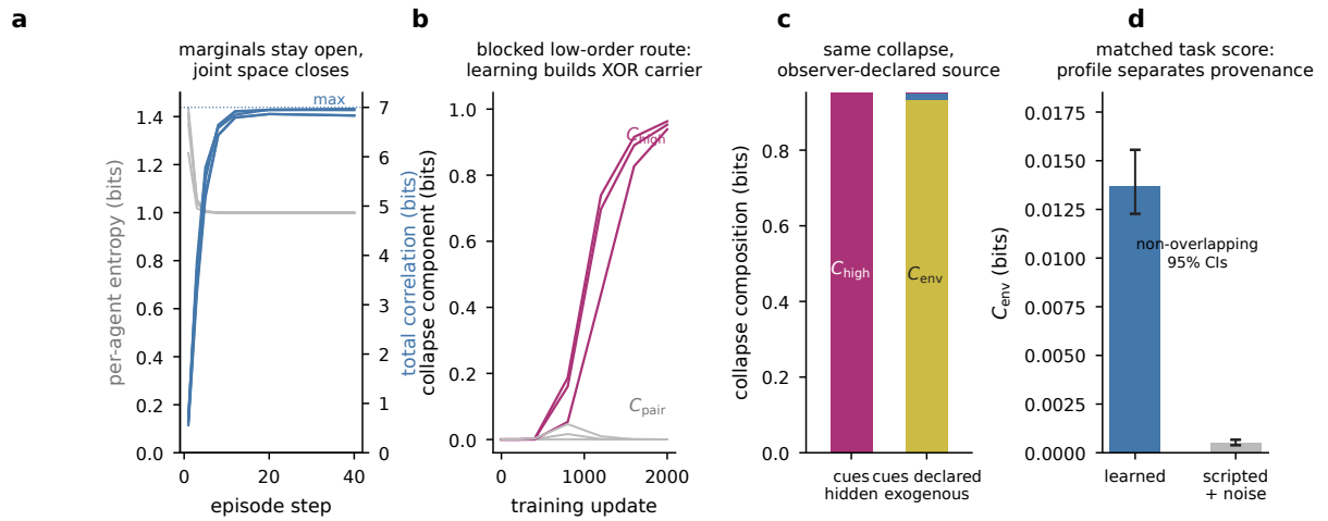
Figure 4. The source typology transfers to learning. a , Hidden-coordination task: per-agent entropy stays open while total correlation rises to near the 7-bit maximum—a purely relational collapse. b , With the low-order route blocked, learning builds an irreducible higher-order (XOR) carrier: C_{high} grows while C_{pair} stays near zero. c , Contract-relativity on the learned system: declaring the private cues exogenous re-attributes the identical collapse from C_{high} to C_{env} . d , At matched task score, the environment-conditioned component separates a learned pair from a noise-matched scripted pair (non-overlapping 95% confidence intervals).
