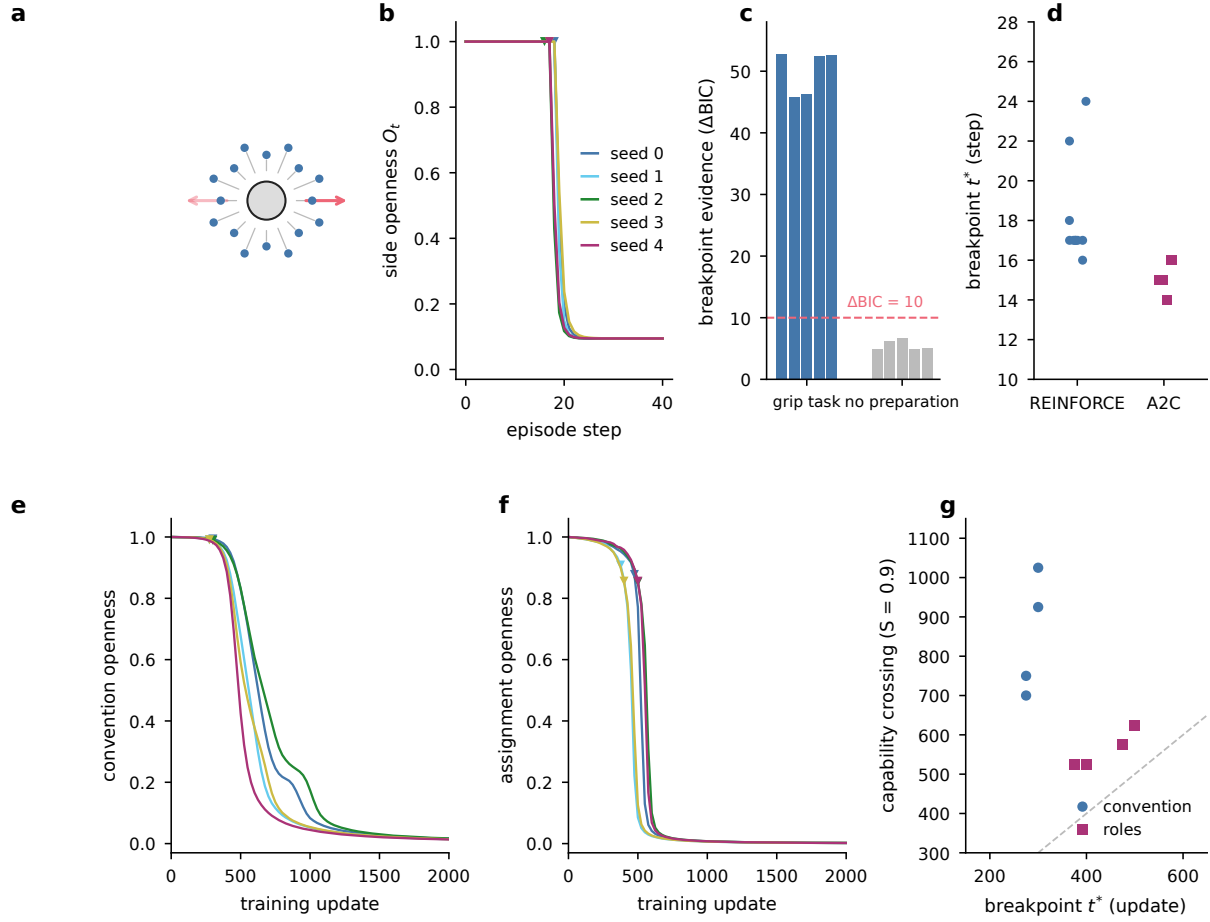
Figure 2. Punctuated commitment in learned collectives. a , The grip-then-push transport task ( N = 16 ): agents must jointly grip before the object can be pushed (arrows, the two possible push directions), structurally delaying the choice of side. b , Side-openness of the joint policy holds on a plateau and then collapses; triangles mark the fitted breakpoint t^* (5 REINFORCE seeds). c , Mechanism contrast: the grip task shows a breakpoint in 5/5 seeds ( \Delta BIC well above 10) whereas a matched no-preparation task shows none (0/5). d , Breakpoint location across seeds and algorithms: 10/10 for REINFORCE, and a partial replication under A2C (5/5 shape and primary hinge, 3/5 strict). e , A ten-agent signalling population with 120 exactly equivalent codes and no gate holds a flat open plateau, then commits with an onset breakpoint (4/5 seeds; triangles), each seed to a different code. f , Six agents locking into a division of labour among 720 equivalent role permutations (5/5 onset, five distinct permutations). g , In all nine onset seeds the possibility-space breakpoint precedes the capability crossing ( S = 0.9 ): commitment is measurable before the ability is expressed.
