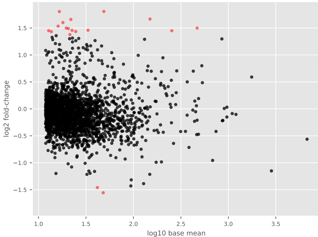
AS vs. control - MA plot
