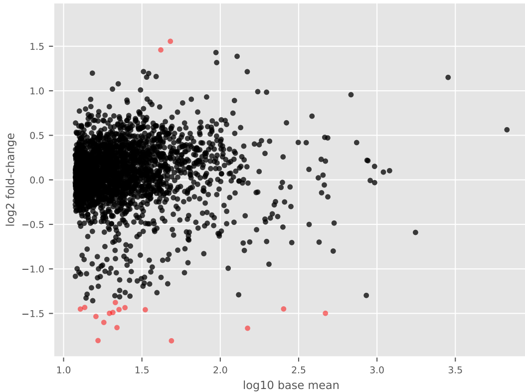
control vs. AS - MA plot
