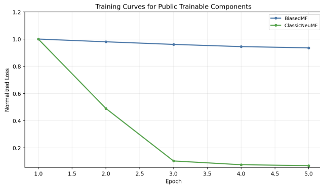
Figure 4: Training loss curves for the public trainable components. The vertical axis is zoomed to the observed range with a 20% margin so the relative convergence behavior is visible.
