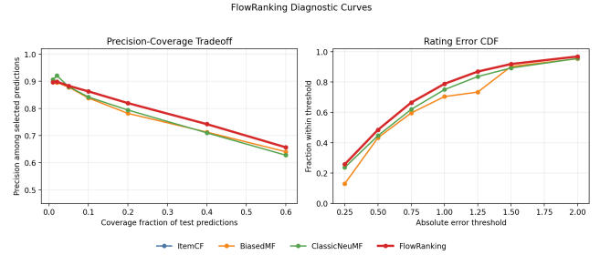
Figure 4: Diagnostic curves for the final recommendation system. The left panel shows the precision–coverage tradeoff for high-confidence predictions, and the right panel shows the cumulative distribution of rating errors. These views complement the metric bar charts by showing how reliability changes with recommendation coverage and error tolerance.
