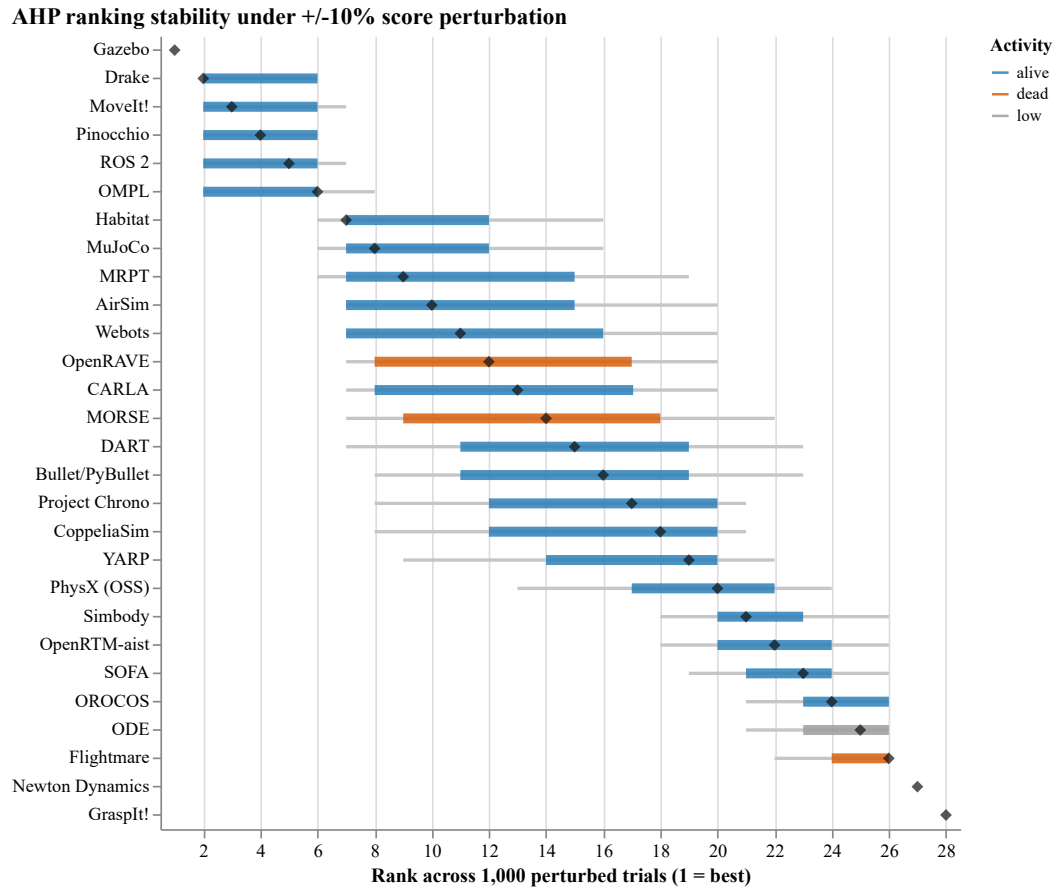
Figure 5.5: Stability of the equal-weight AHP ranking under a \pm 10\% score perturbation. Diamond, baseline rank; thick bar, 5th–95th percentile; thin line, full range.
