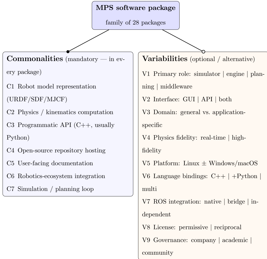
Figure 4.1: Commonality/variability feature model for the 28-package MPS software family. Filled circle (●) marks the mandatory features shared by every package; open circle (○) marks optional or alternative features. Commonalities C1–C7 are described in Section 4.3; variabilities V1–V9 and their binding times appear in Section 4.4 and Table 4.1.
