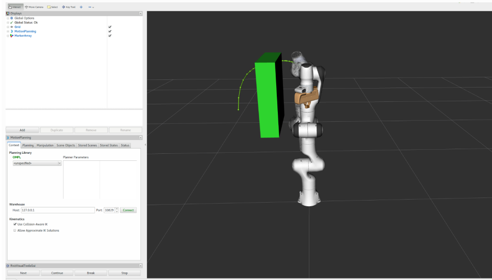
Figure 1.1: A manipulator planning a collision-free trajectory around an obstacle: an illustrative motion planning task.
