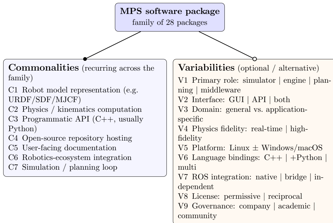
Figure 4.1: Commonality/variability feature model for the 28-package MPS software family. A filled circle (●) marks commonalities; an open circle (○) marks variabilities. Commonalities C1–C7 are detailed in Section 4.3; variabilities V1–V9 and their binding times in Section 4.4 and Table 4.1.
