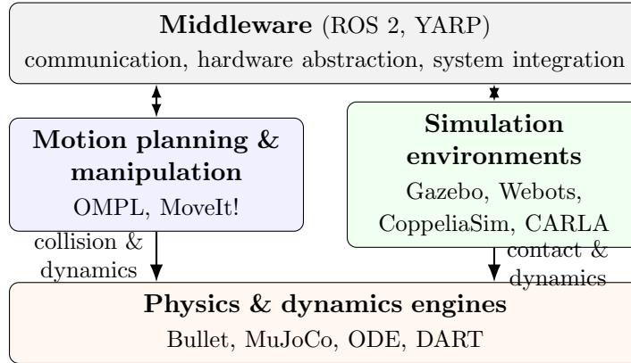
Figure 2.1: Representative software roles in a motion planning and simulation workflow and how they interact. Simulation environments and planning or manipulation stacks both build on shared physics and dynamics engines (downward arrows: contact, collision, and dynamics queries), while middleware wires the functional components together (double arrows: messages, services, and hardware abstraction). The packages named in each box are illustrative examples from this report’s selected set; many tools span more than one role, as discussed in Chapter 4.
