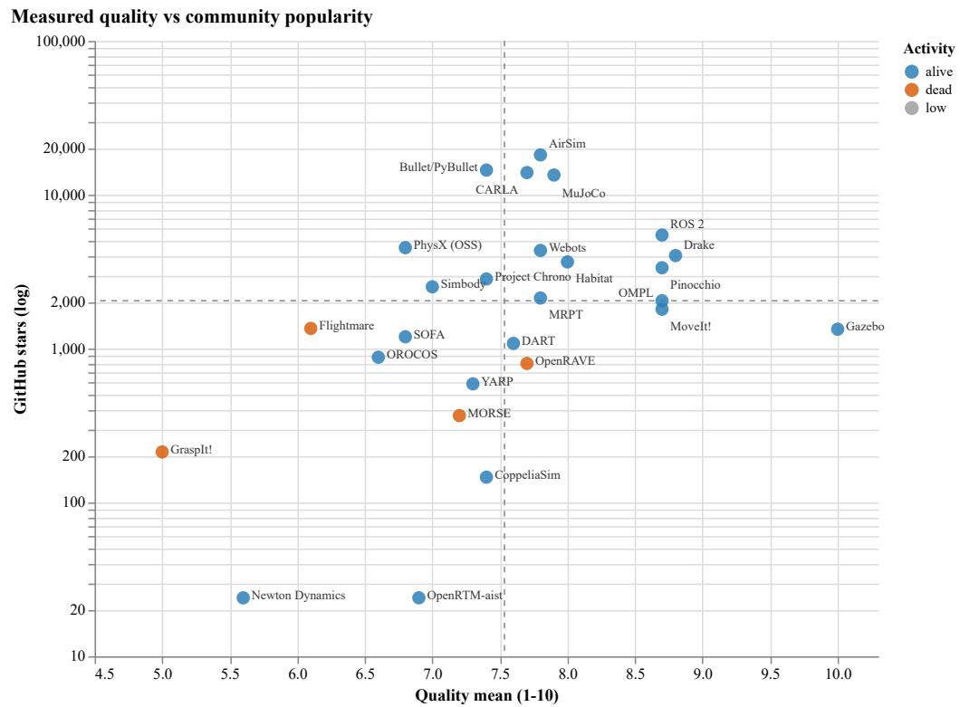
Figure 5.7: Measured quality mean versus GitHub stars (log scale) for the 28 packages, coloured by the 18-month repository-activity flag (Section 3.5.3). Dashed lines mark the mean quality and the median star count.
