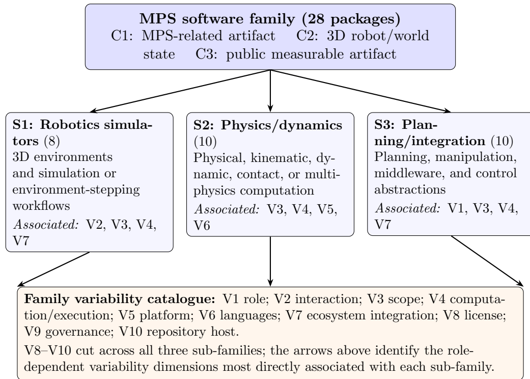
Figure 4.1: Relationship between the MPS family, its three role-based sub-families, and the ten variability dimensions. The sub-family boxes identify their most direct role-dependent variabilities; V8–V10 apply across all three groups.
