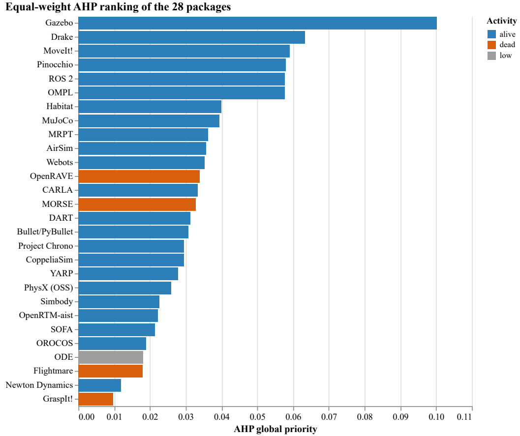
Figure 5.3: Equal-weight AHP global-priority ranking ( c_k = 1/9 ) of the 28 packages.
