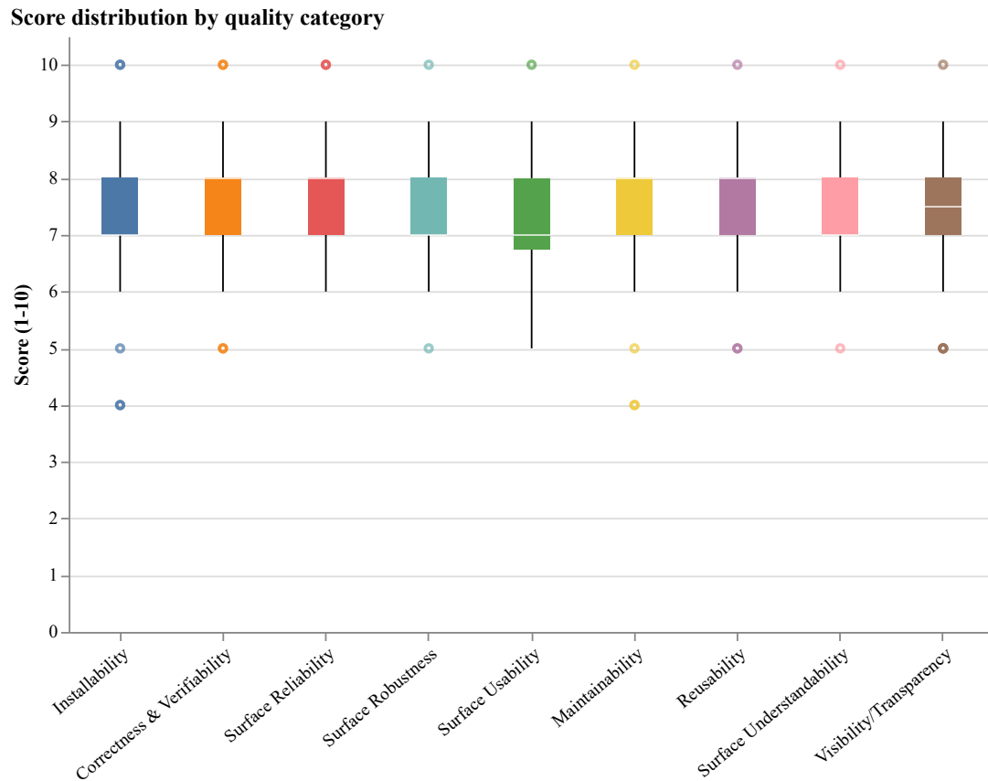
Figure 5.2: Distribution of the impression scores across the 28 packages within each of the nine quality categories (box plots).
