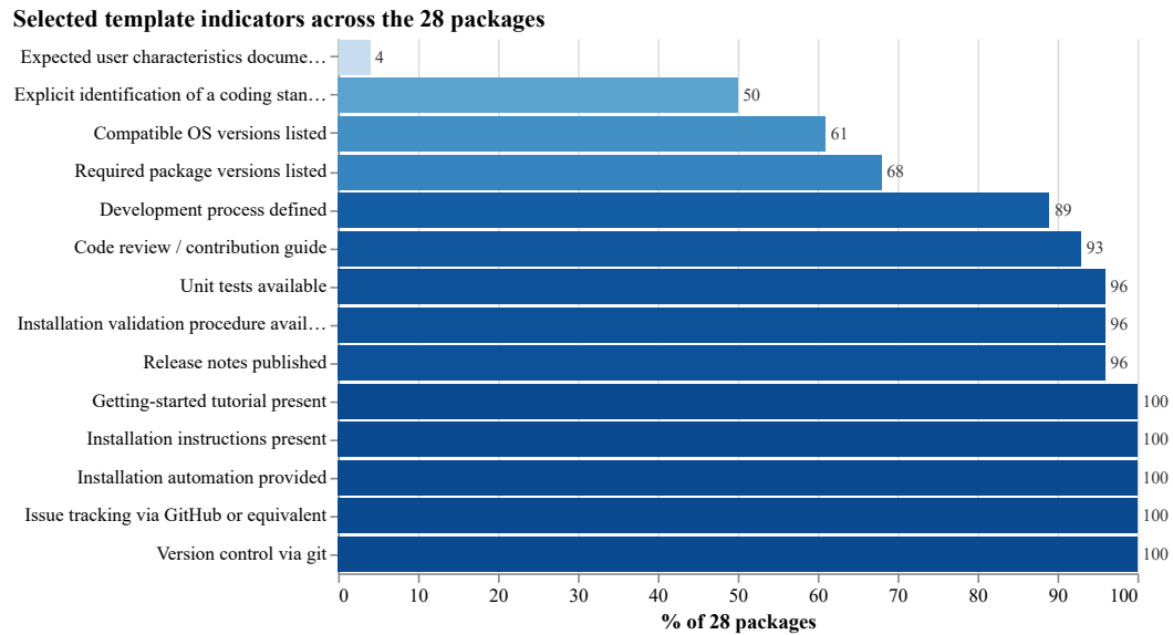
Figure 5.5: Coverage of selected measurement-template indicators across the 28 packages, sorted from least to most common.
