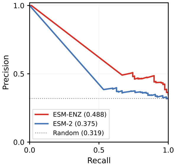
EC Classification
