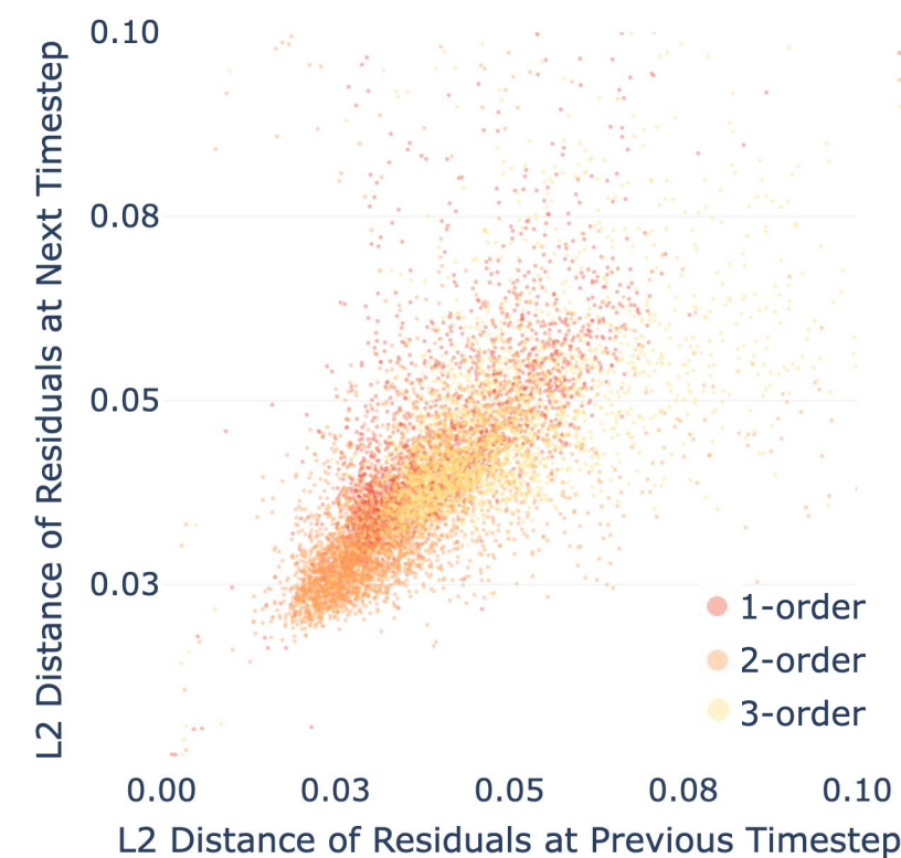
(e) Intra-Cluster Residual Relationships across Timesteps
