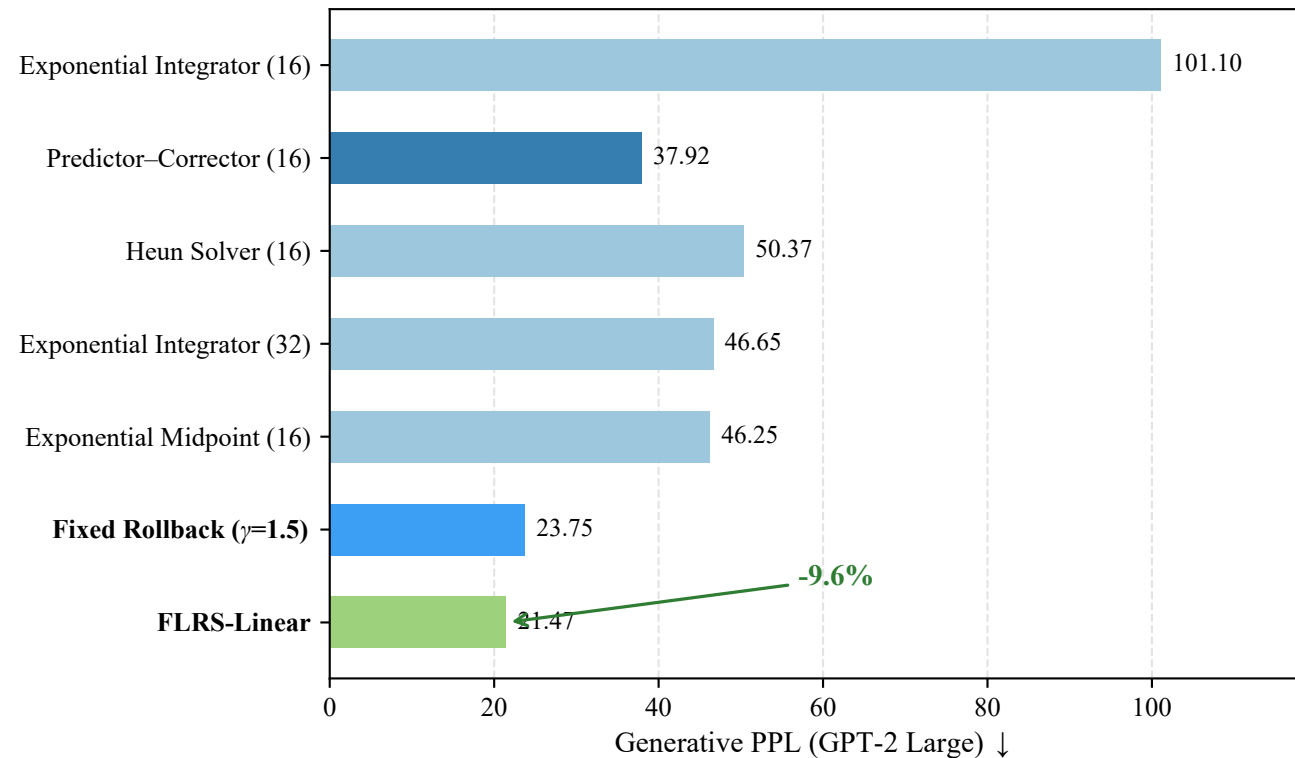
(a) 32-NFE budget
