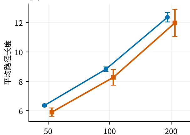
(a) TSP ↓
