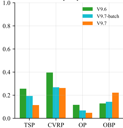
Search-step improve rate
