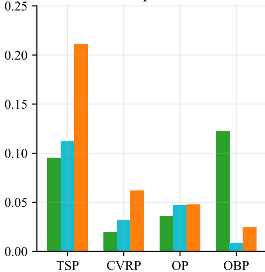
Search-step invalid rate
