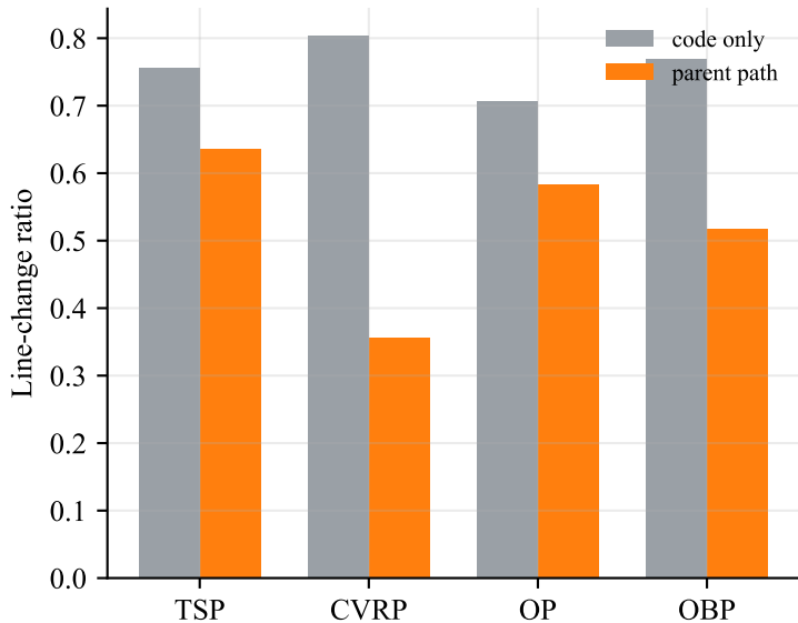
Modification magnitude
