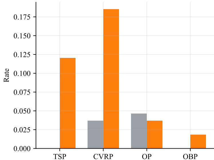
Parent-improvement rate
