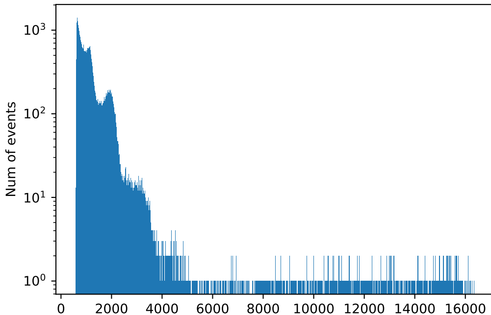
Bi207 peak max, channel no. 01, at 1300V
