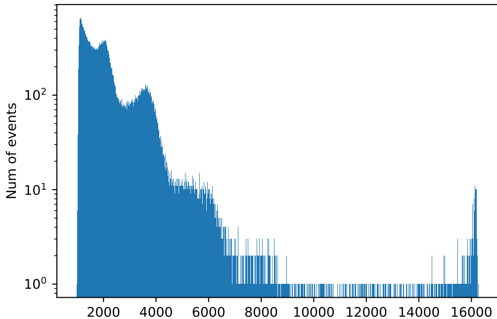
Bi207 peak max, channel no. 07, at 1300V
