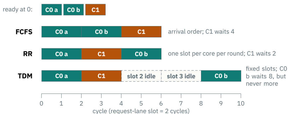
Figure 8.3. Three requests ready at the same cycle on one request lane — two from core 0, one from core 1 — under the three shipped arbiters.
