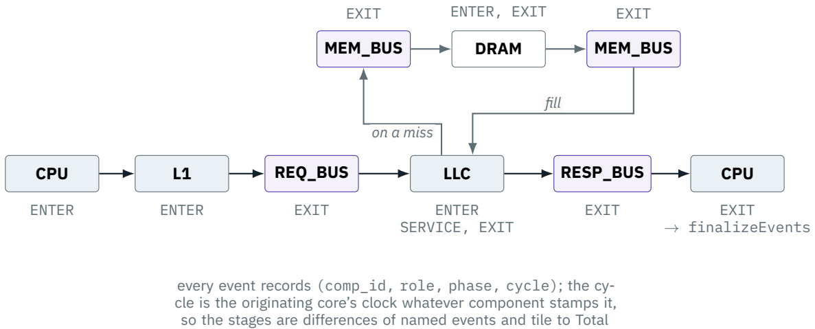
Figure 11.1. The Logger's view of one request: a chain of self-describing events.
