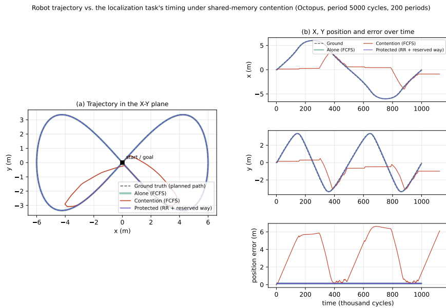
Figure 12.2. The robot's path in the three acts: alone and protected coincide exactly; under contention one 181 266-cycle job left the robot steering for 35 periods on a stale waypoint, the long chord across the figure.
