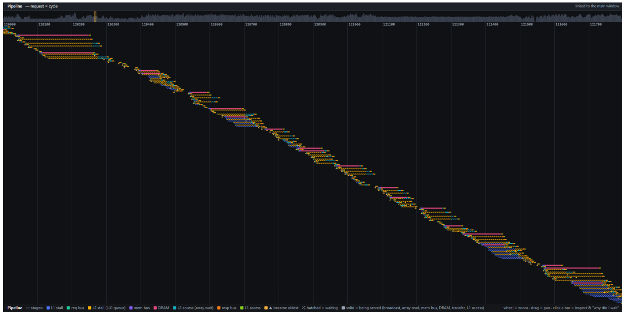
(a) Pipeline: one row per request, one bar per stage, hatched while waiting, solid while served.
