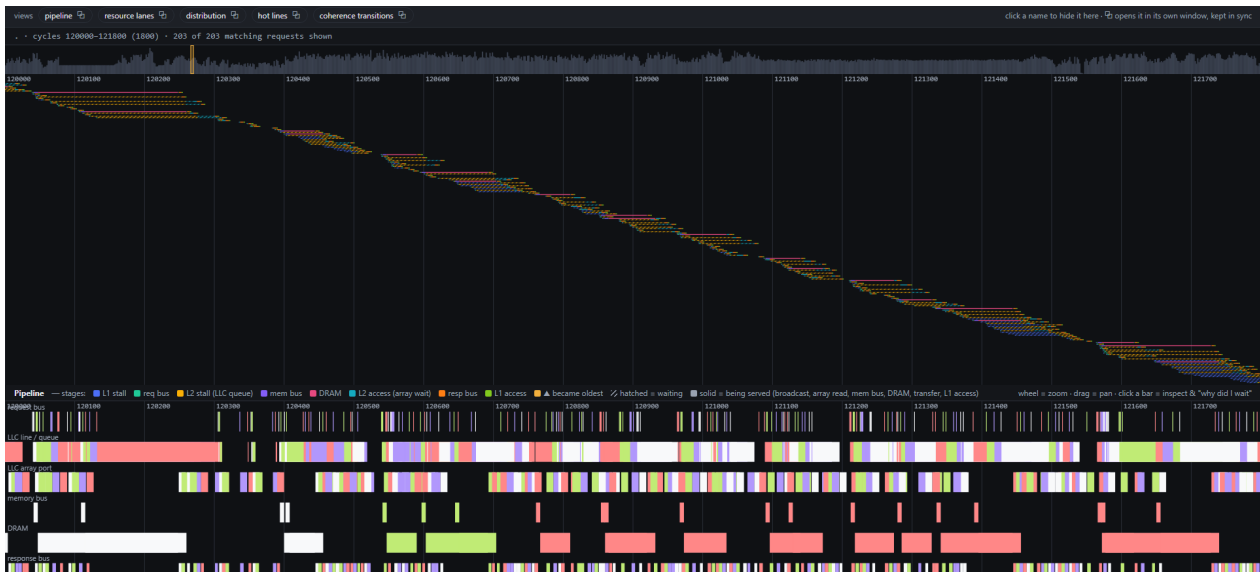
Figure 11.5. The visualizer on cycles 120 000–121 800 of a2time01 : the filter bar and the view tabs on top, the request pipeline (one row per request, one bar per stage, hatched while waiting) and, below it, the resource lanes (the same cycles seen from each shared resource, coloured by the core that held it).
