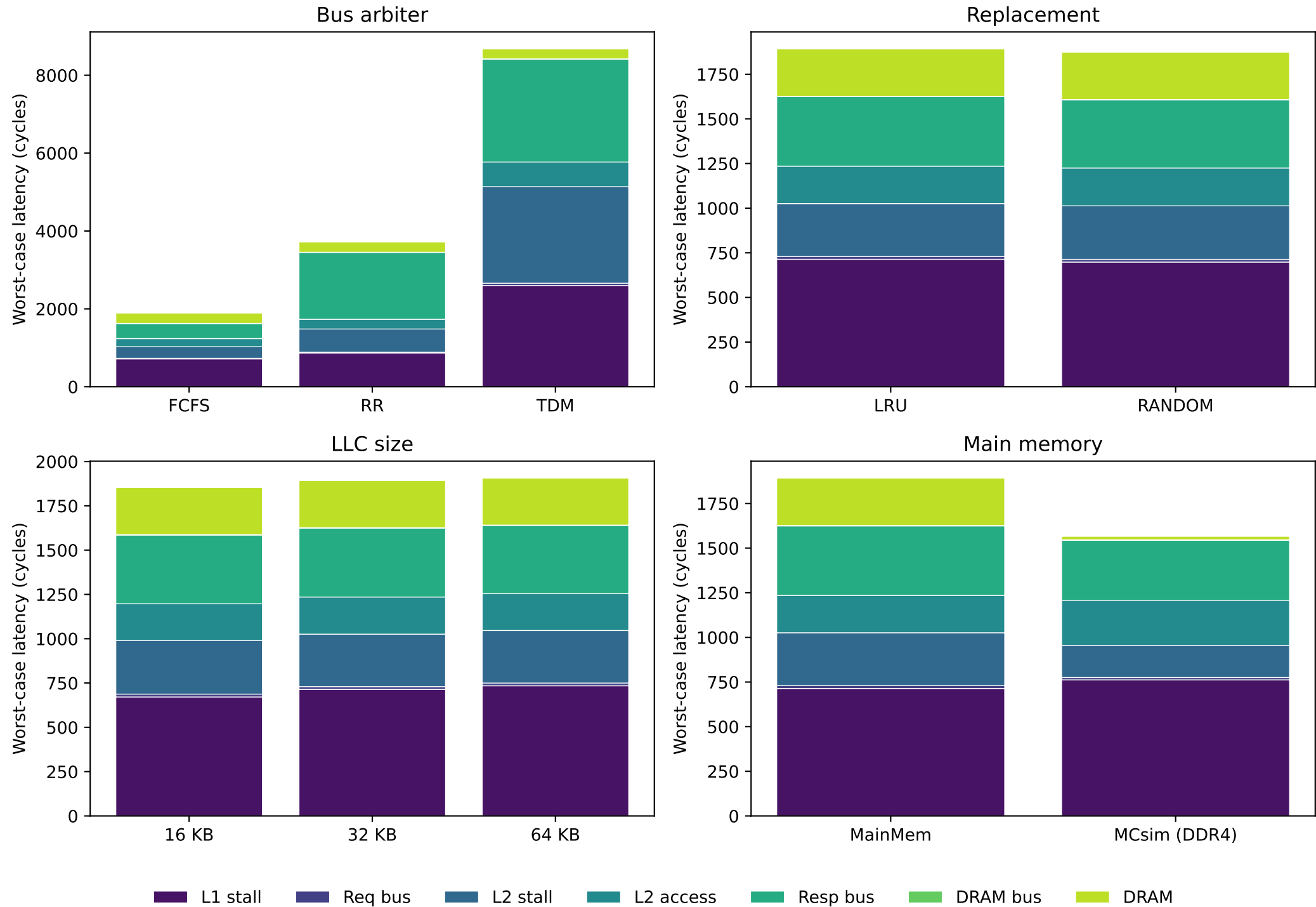
Worst-case latency, decomposed by pipeline stage (EEMBC, mean over benchmarks)
