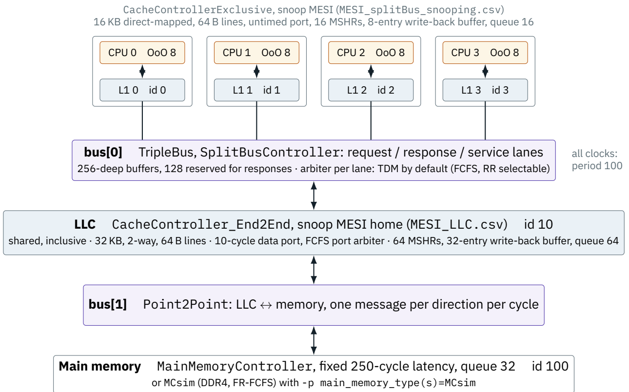
Figure 3.4. The system MultiCoreSystem.csv builds. Four trace-driven cores with private MESI L1s on a TripleBus, one shared inclusive LLC, a point-to-point memory bus and a fixed-latency main memory. Every number is a configuration key (Chapter A).
