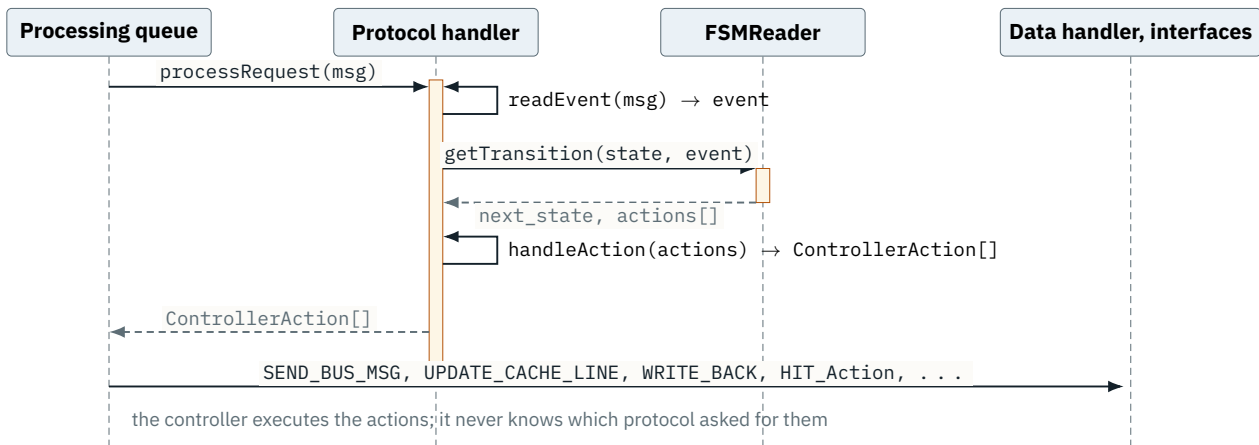
Figure 4.2. One message through the controller. The handler decodes the message into an event, looks up the transition for the line's current state, and hands the controller a list of protocol-agnostic actions; the controller does not know which protocol it is running.
