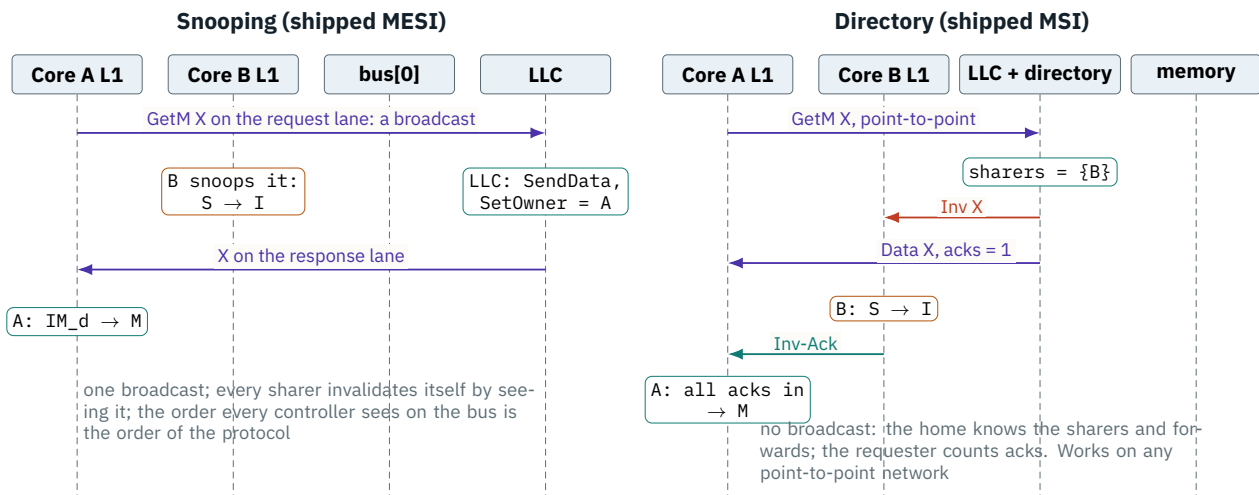
Figure 6.2. One GetM from core A while core B shares the line, under the shipped snooping MESI (left) and the shipped directory MSI (right).
