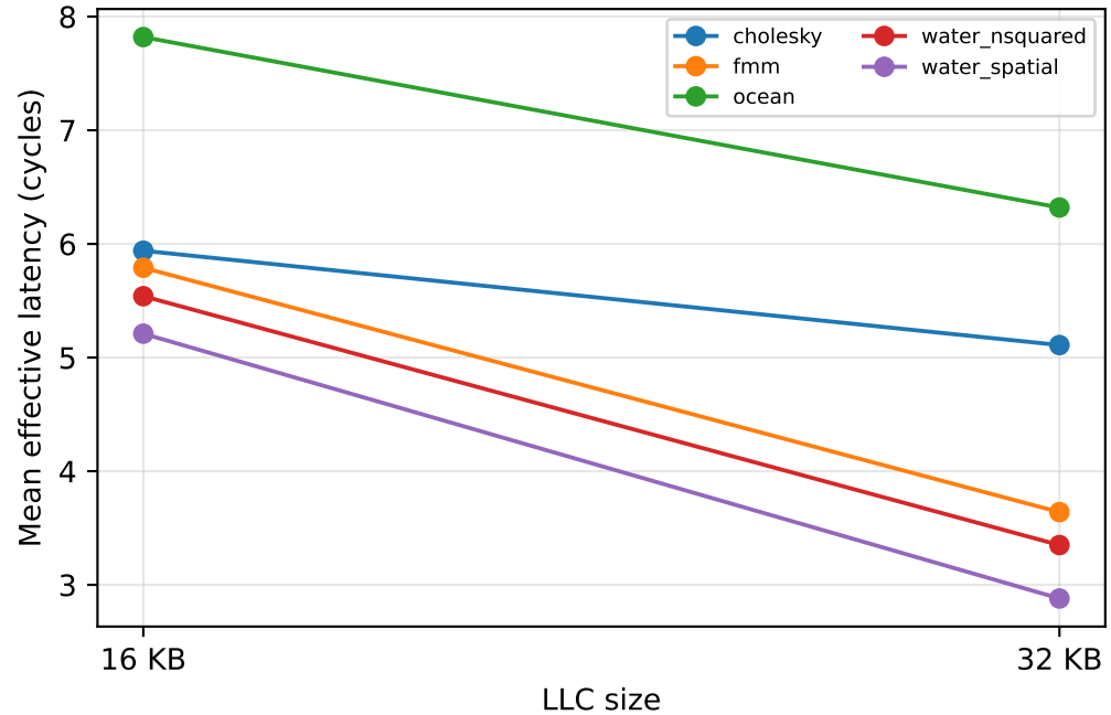
SPLASH
