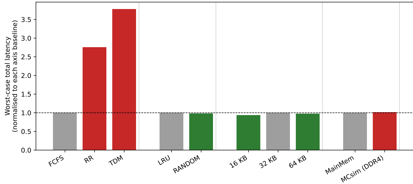
Every axis moves the needle — WCET relative to baseline (EEMBC)
