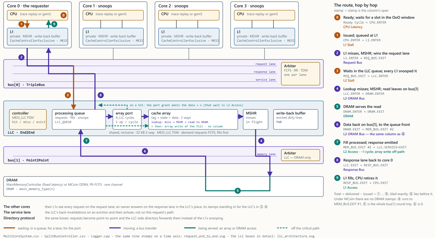
Figure 7.1. The system as shipped with one LLC miss from core 0 routed through it. Each hop carries the colour of the LatencyReport column that measures it (amber: waiting; purple: a bus transfer; teal: being served) and the number of the Logger stamp that bounds it, ①–⑩ being the report's nine latency columns in order; the side panel lists the stamp pair behind every column.
