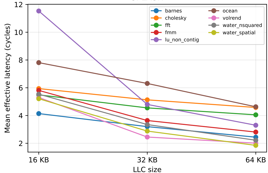
SPLASH
