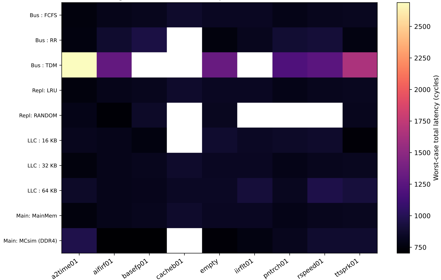
Configuration x benchmark response surface (EEMBC wcTotal)
