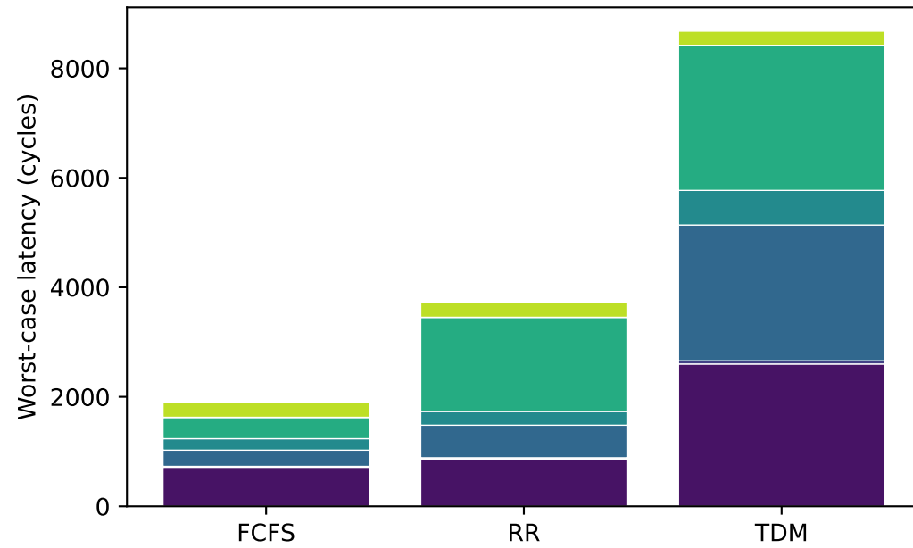
LLC size
