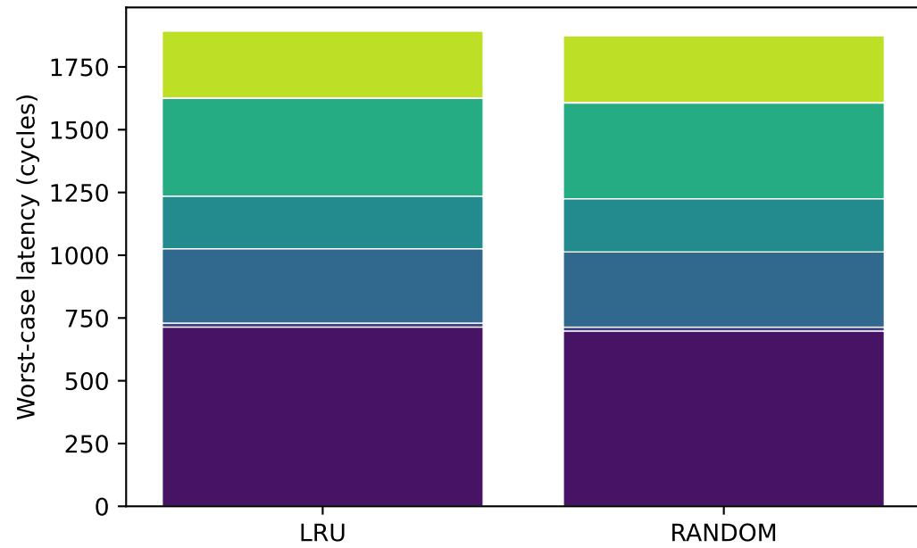
Main memory
