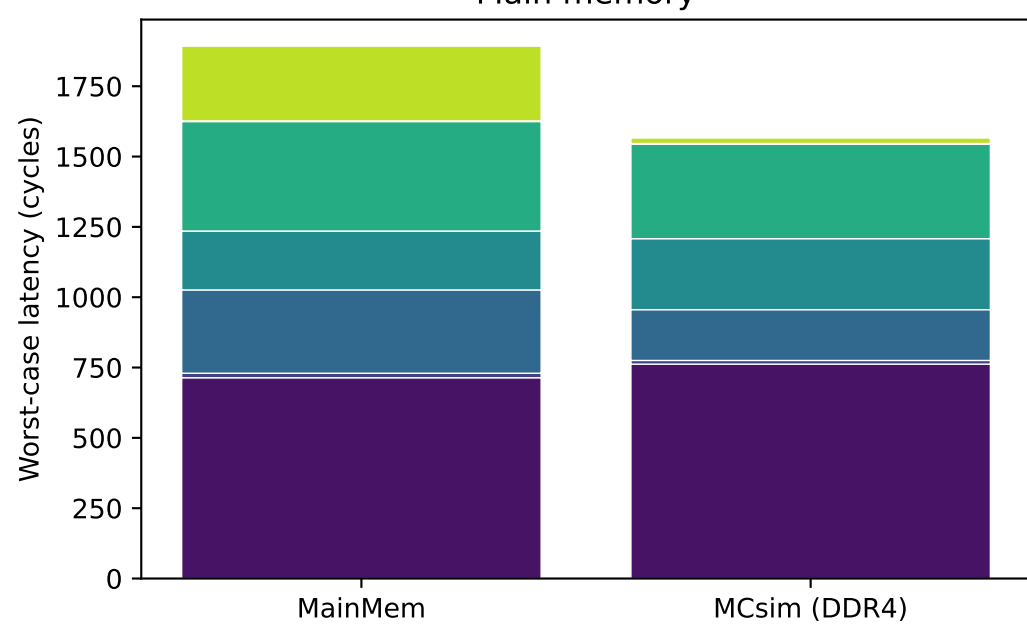
Main memory
