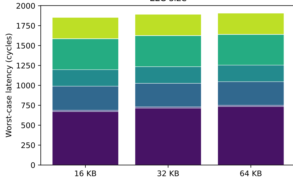
LLC size
