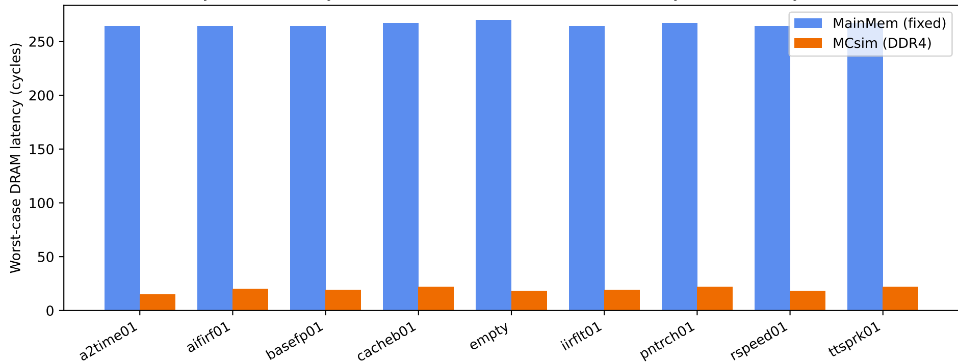
Memory-model axis: cycle-accurate MCsim DDR4 vs fixed-latency main memory (EEMBC)
