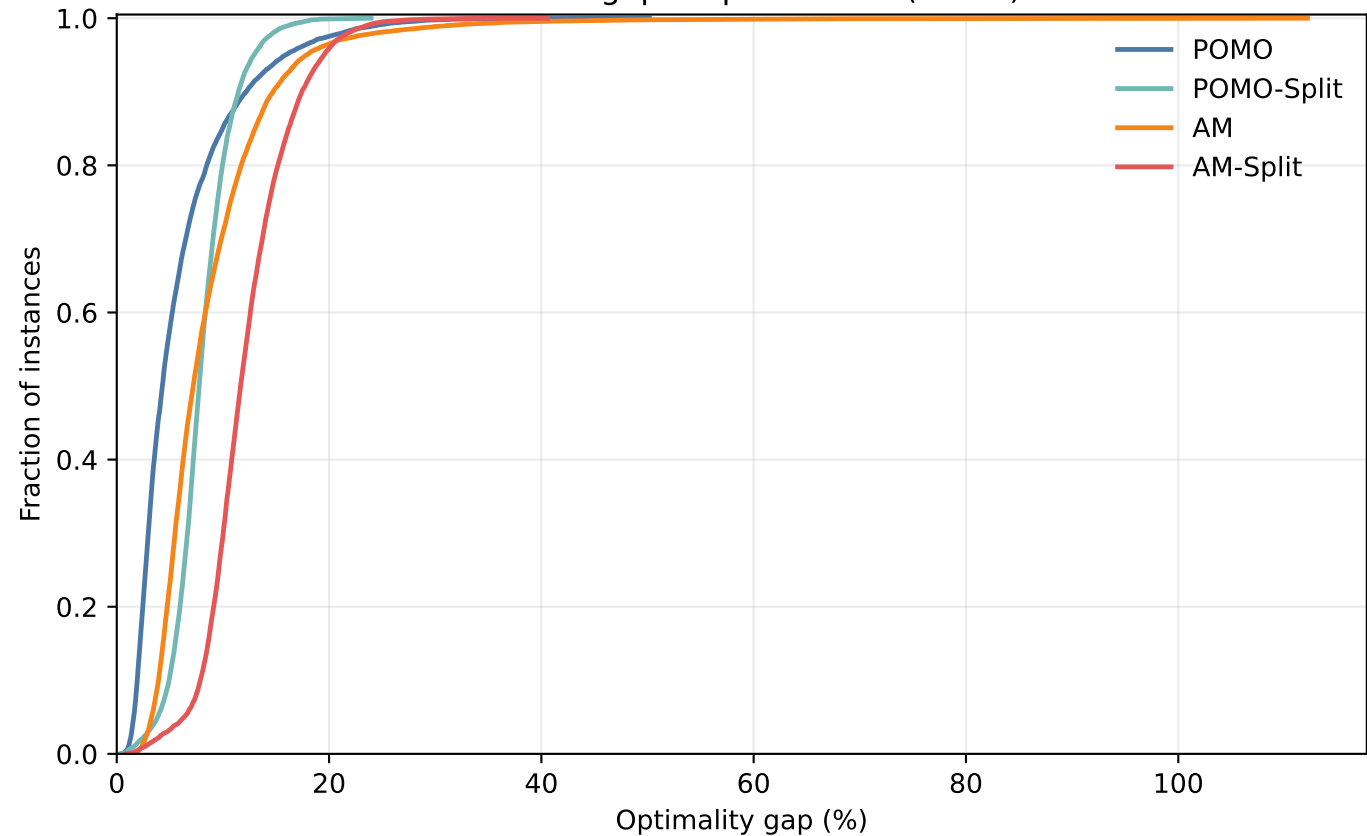
XML100 gap empirical CDF (8-fold)
