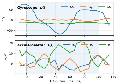
IMU Measurements
