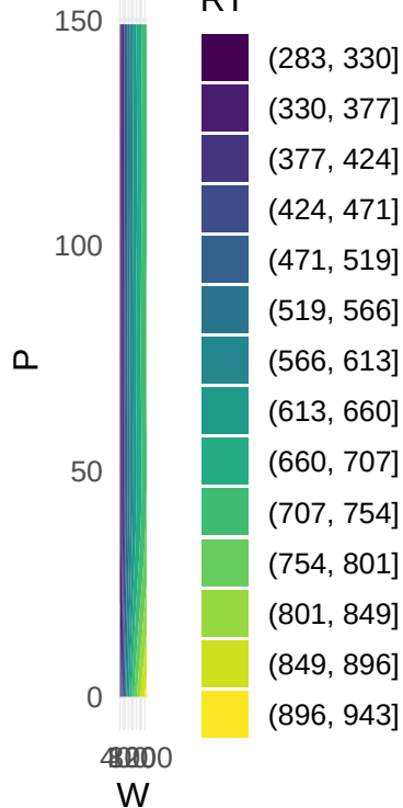
P & W (GAM)
