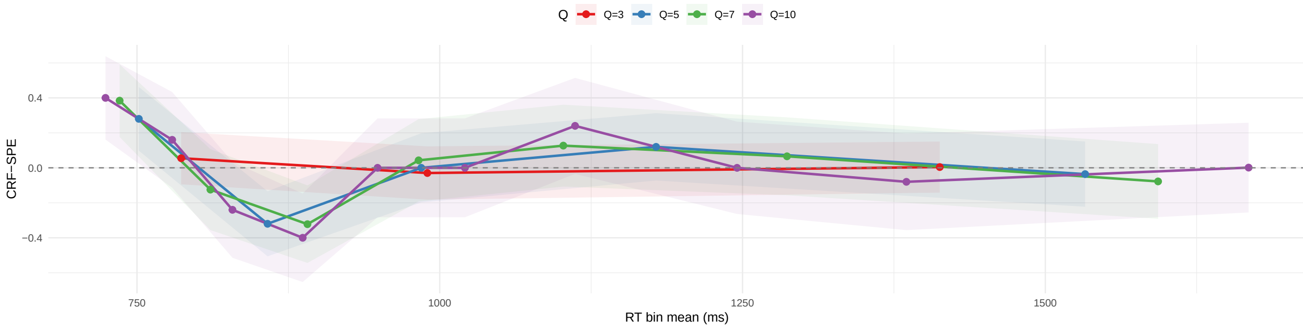
G6-S3: CRF-SPE across Quantiles
