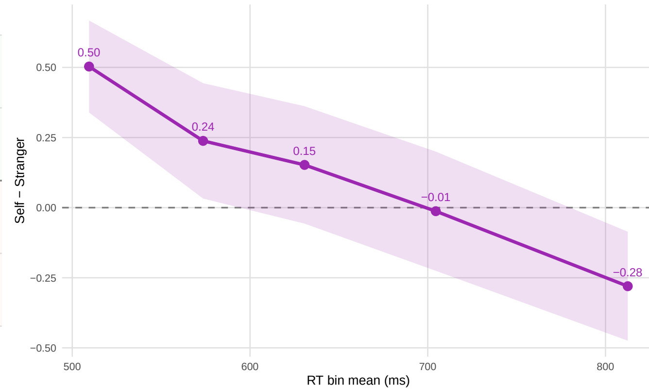
CRF-SPE
