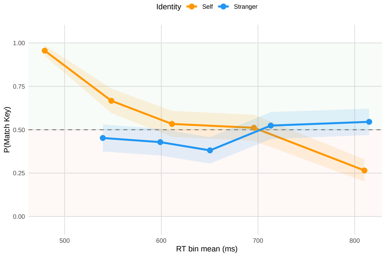
G8-S4: CRF-SPE across Quantiles
