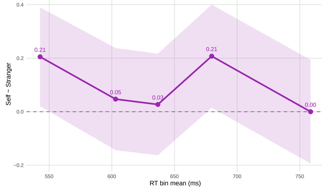
CRF-SPE
