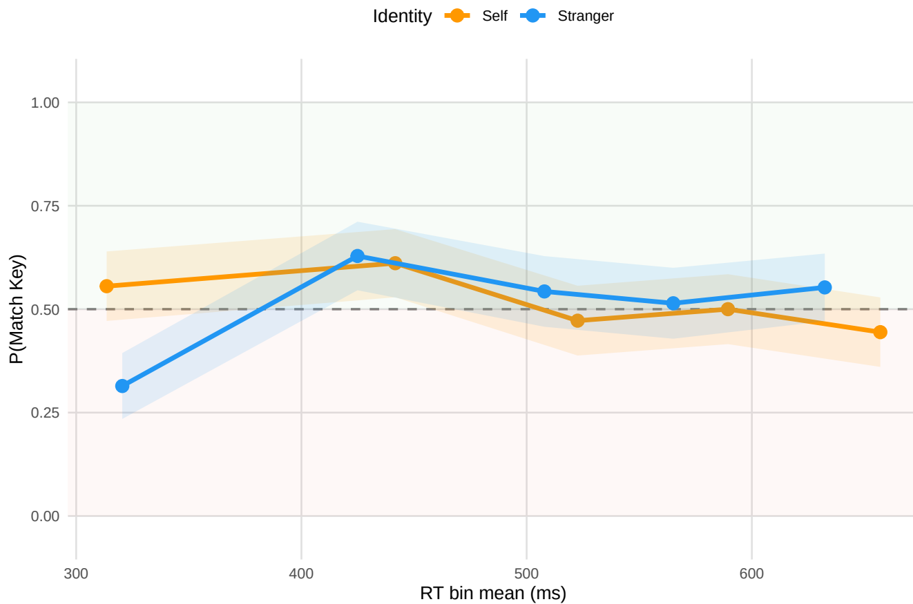
G4-S1: CRF-SPE across Quantiles
