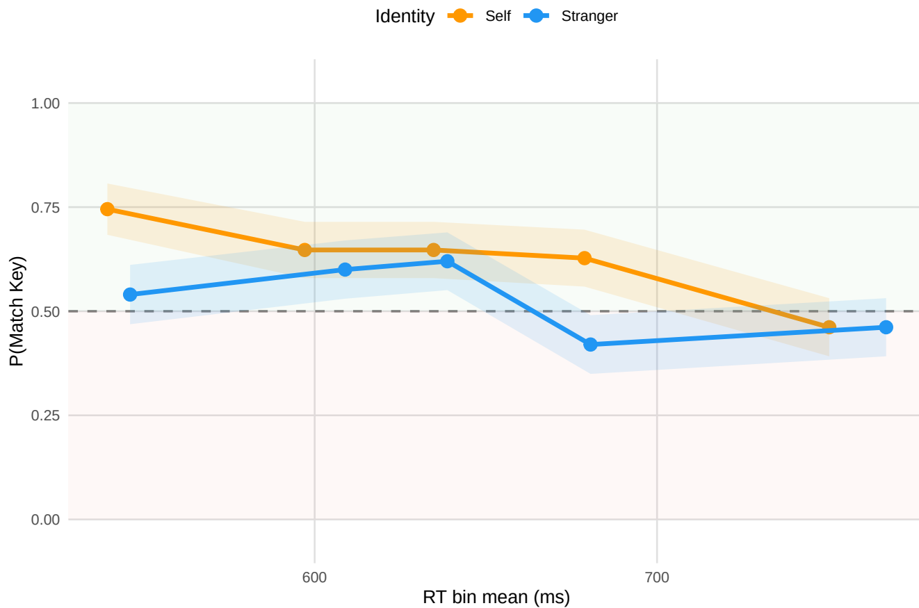
G8-S10: CRF-SPE across Quantiles
