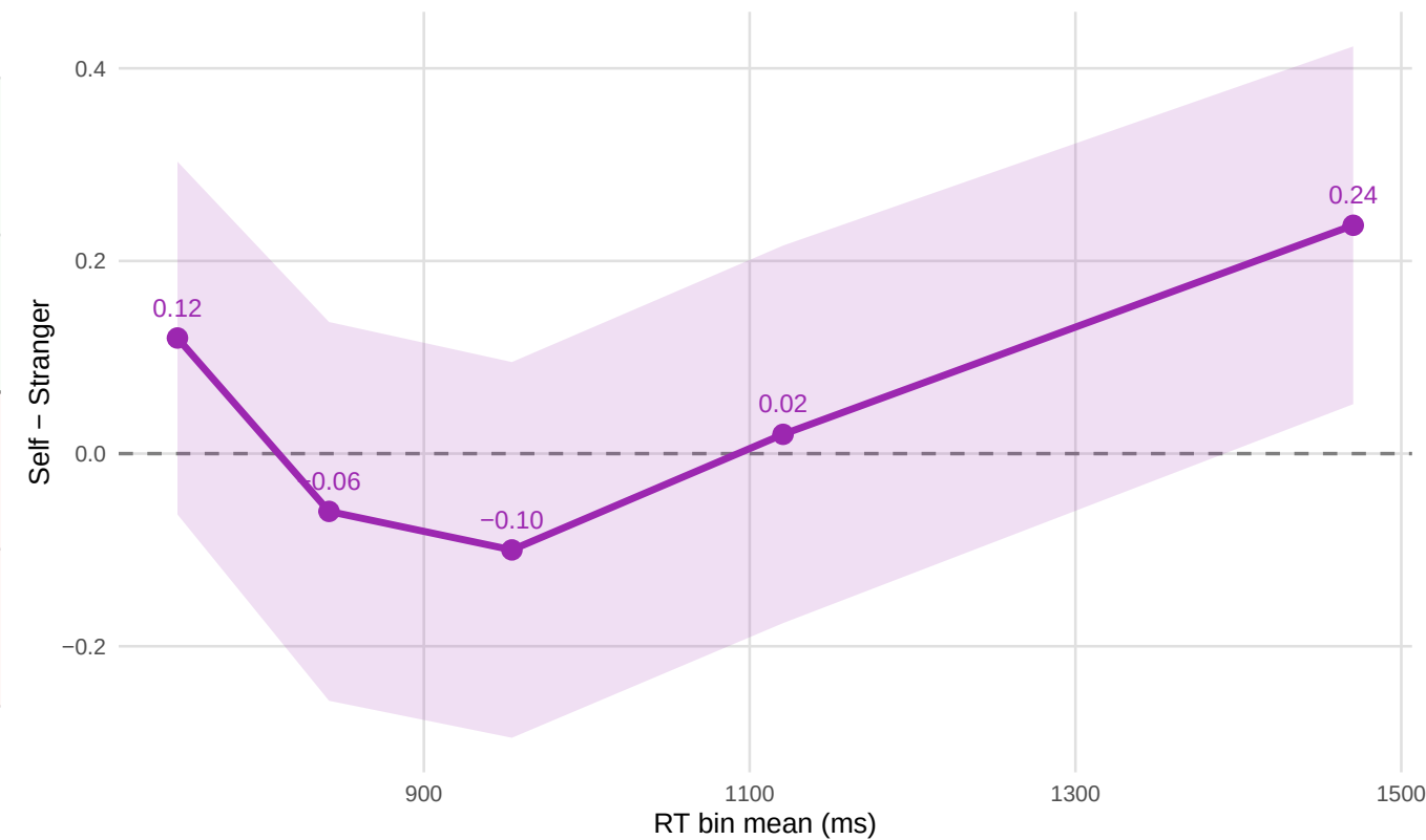
CRF-SPE
