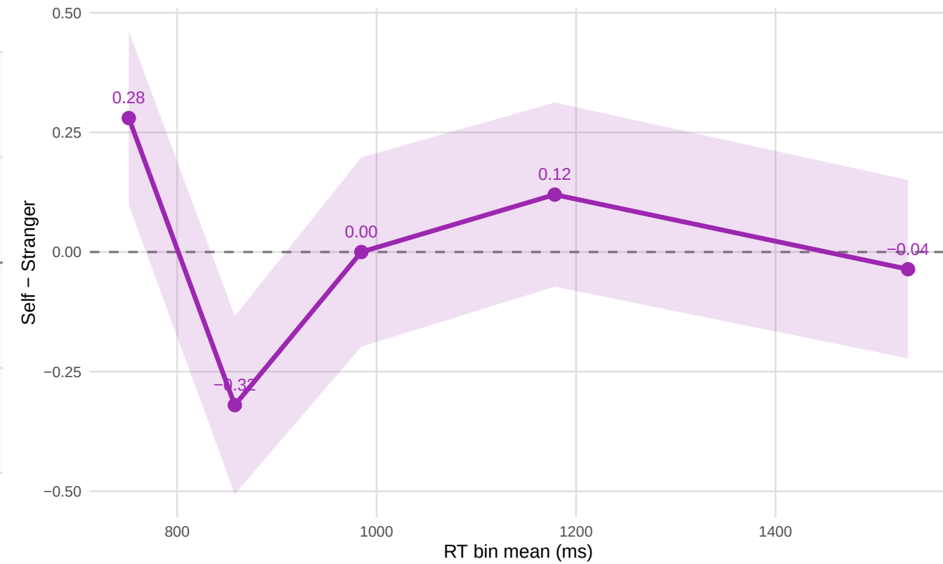
CRF-SPE
