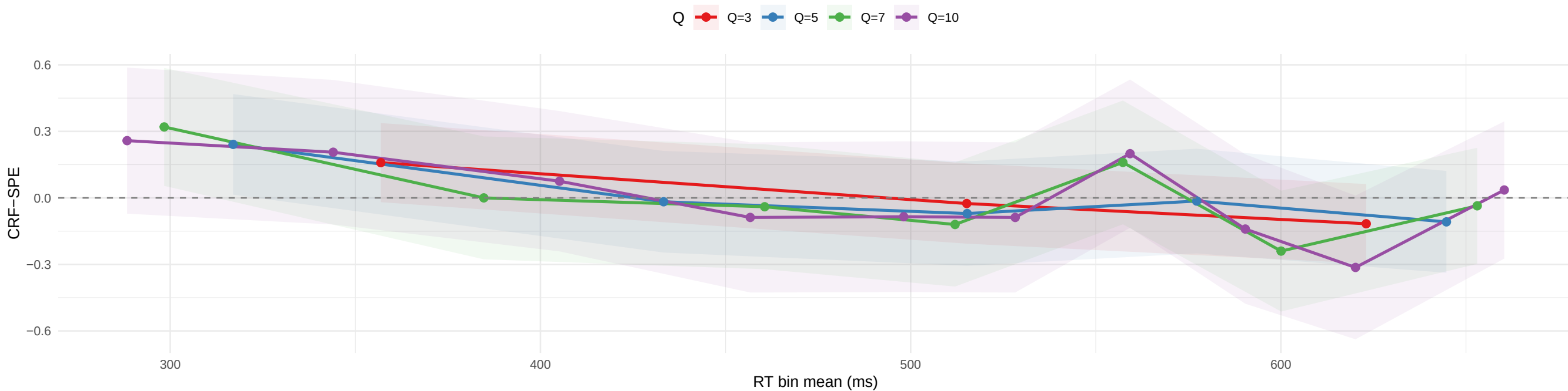
G4-S1: CRF-SPE across Quantiles
