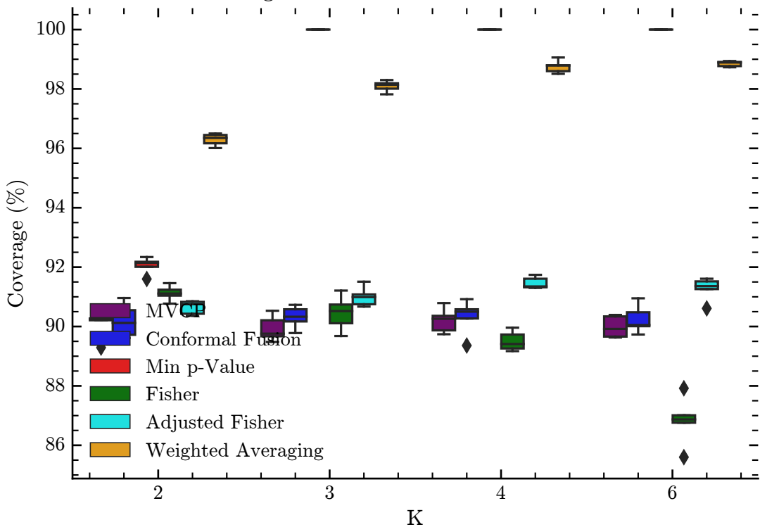
Coverage vs. Number of Views on CIFAR-100
