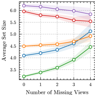
Set Size vs. Missing (K=6)
