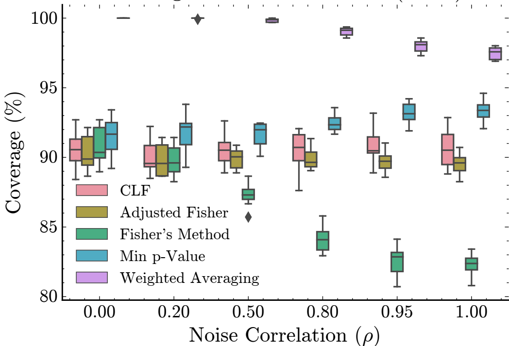
Coverage vs. Noise Correlation ( K=6 )
