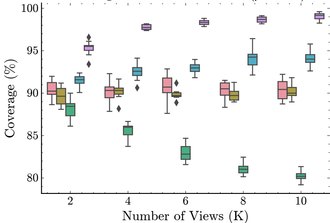
Coverage vs. Number of Views ( \rho=0.90 )
