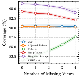
Coverage vs. Missing (K=6)
