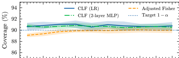
CIFAR-100 (K=4): Coverage vs n_{\text{fuse}}/n_t
