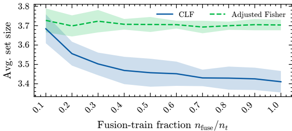
Set size vs n_{\text{fuse}}/n_t
