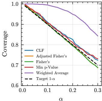
Coverage vs \alpha
