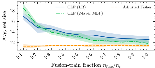
CIFAR-100 (K=4): Set size vs n_{\text{fuse}}/n_t
