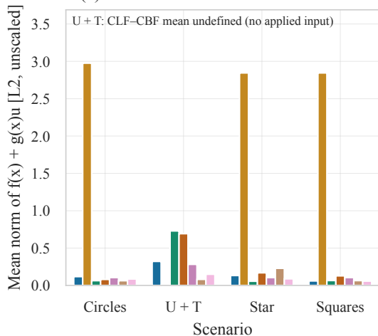
(a) Mean actual state-derivative norm
