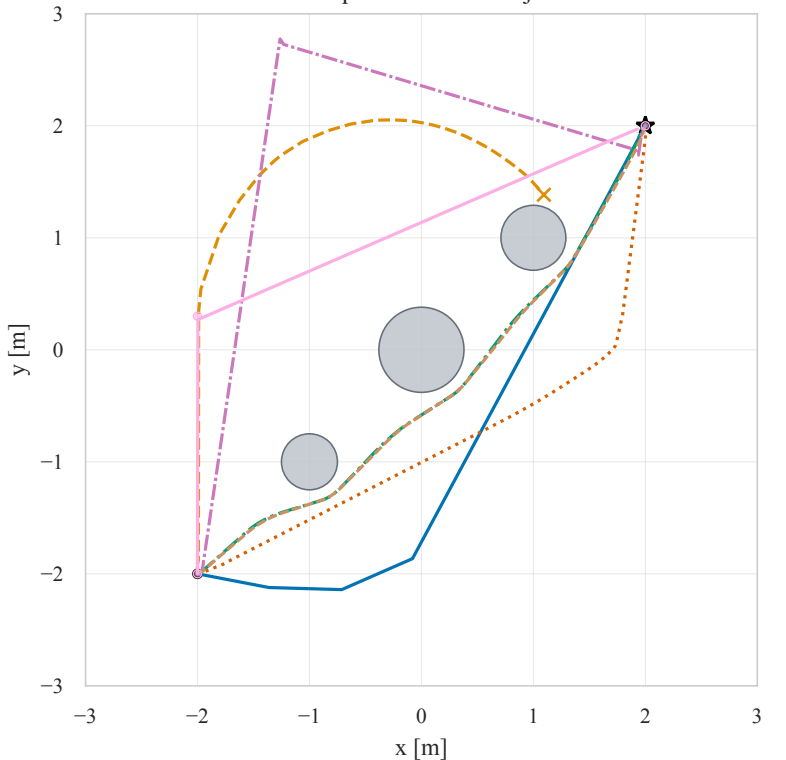
Three unequal circles — trajectories
