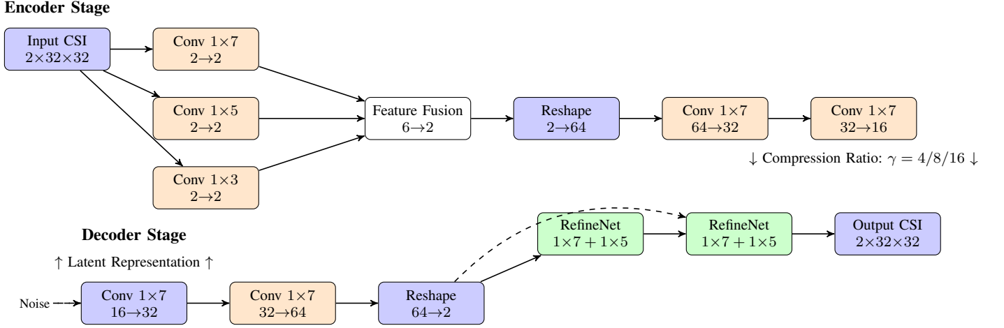
Fig. 2: Complete CLLWCsiNet architecture: (Upper) Encoder stage with multi-scale feature extraction and latent space compression. (Lower) Decoder stage with reconstruction and denoising refinement. The \gamma denotes compression ratio options.
