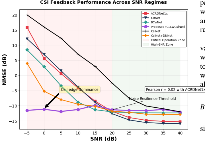
Fig. 3: Performance of Models under the various noise power and compression ratio of 8
